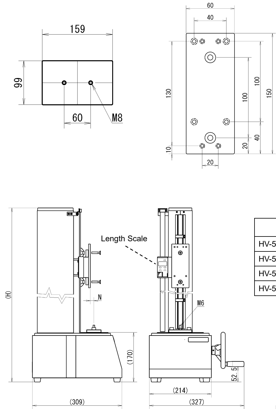
Mounting Plate for Force Gauge
